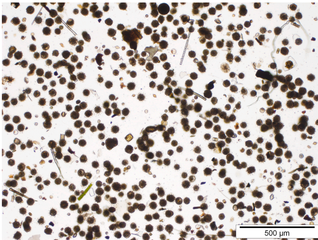
Fig. 16. Light microscope image of cysts from surface sediment from Pornichet Port (PO, 23 February 2022). Scale bar = 500 μm.
