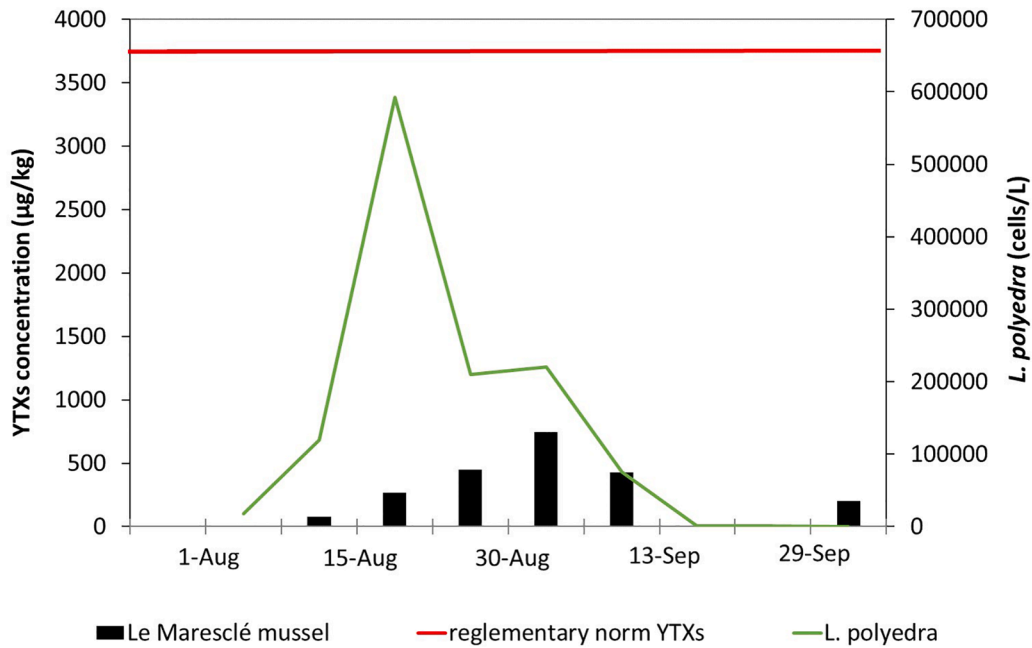
Fig. 13. YTX concentrations measured in mussels in Vilaine Bay (Le Maresclé station, LM) and L. polyedra concentrations (cells/L) from Ouest Loscolo (OL). Reglementary norm is indicated.
