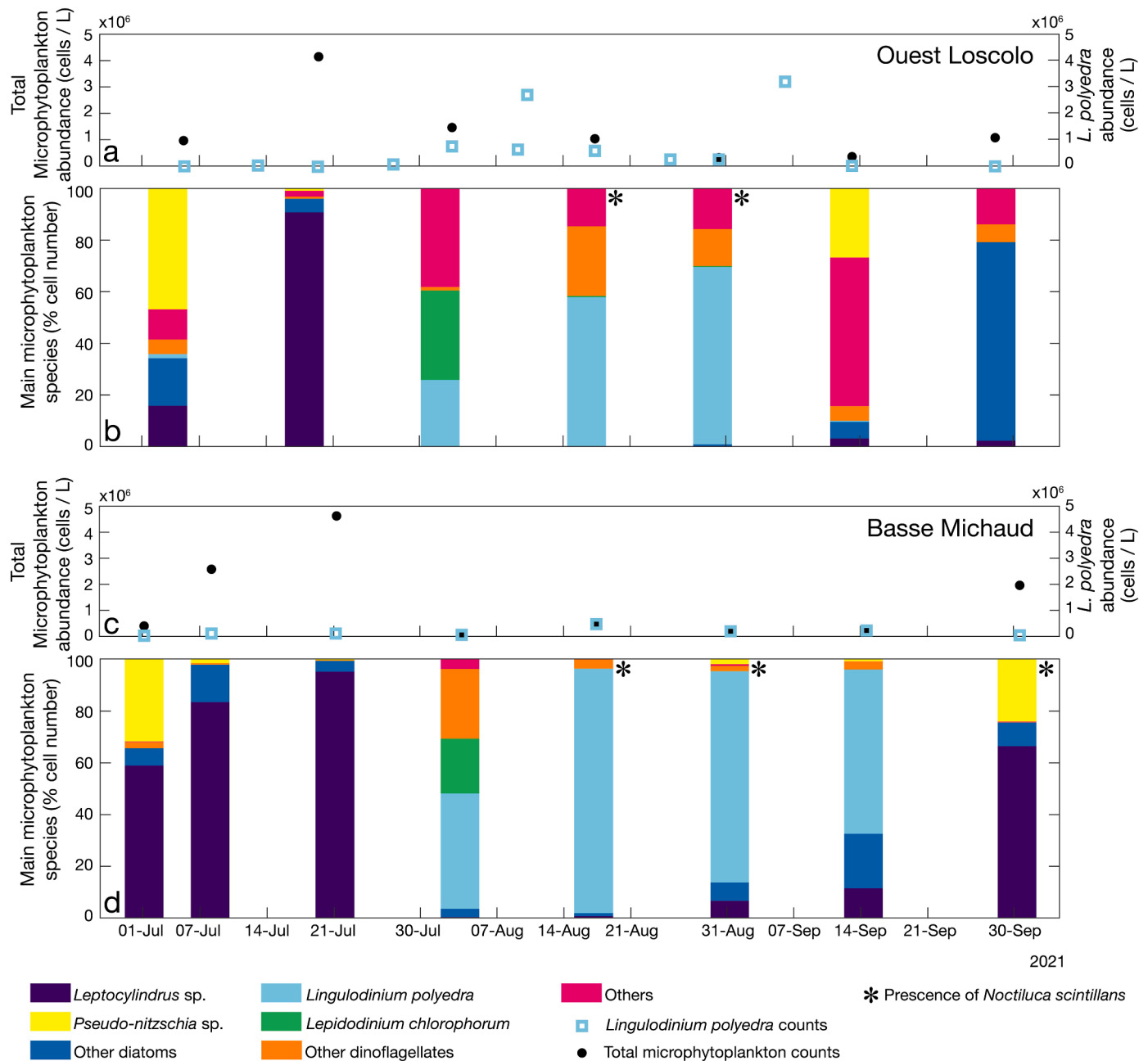
Fig. 2. L. polyedra cell concentrations and assemblage changes in the plankton observed at Ouest Loscolo (OL) (a, b) and Basse Michaud (BM) (c, d) throughout the summer of 2021.
