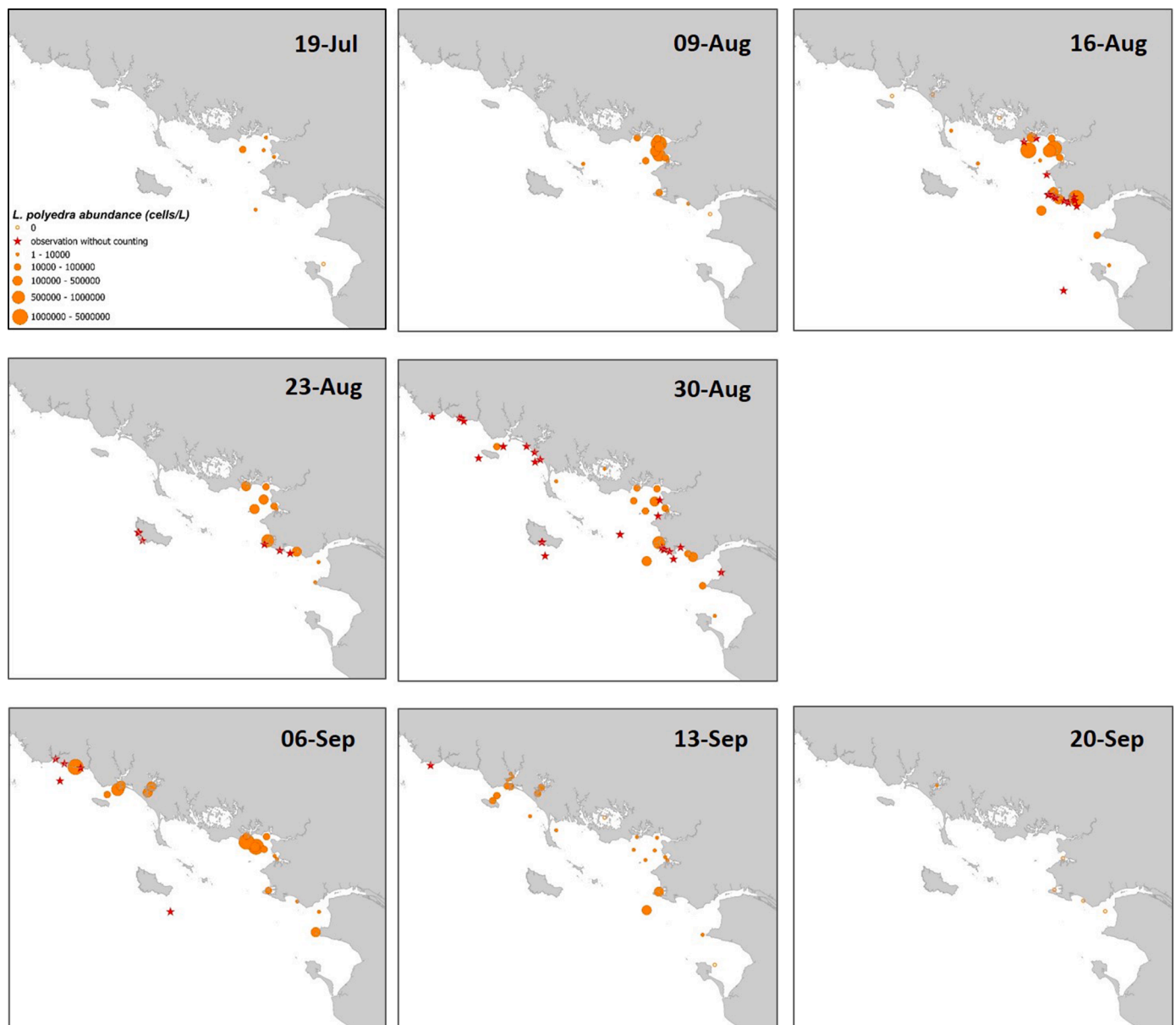
Fig. 3. Spatial and temporal changes of L. polyedra abundances (cells/L) observed within the framework of the REPHY network and the PHENOMER project (red stars largely denote PHENOMER observations).
