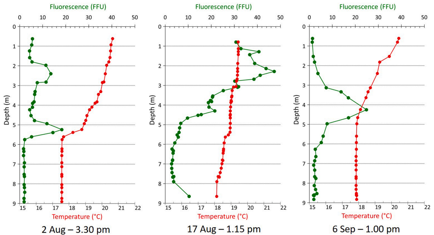
Fig. 9. Fluorescence and Temperature profiles at Ouest Loscolo (OL) on August 2nd, August 17th and September 6th 2021.
