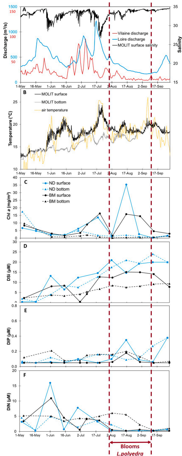
Fig. 8. Variations of environmental parameters from May to September 2021 (A) Variations in daily river discharge ( \text{m}^3/\text{s} ) of the Loire and the Vilaine and salinity recorded at high-frequency by the MOLIT buoy at Nord Dumet (ND) station. (B) Time-series of temperature recorded at high-frequency by the MOLIT buoy at ND station, and air temperature at the weather station Vannes-Séné. (C) Chl a ( \mu\text{g}/\text{L} ) in surface water at ND. (D–F) DSI, DIP and DIN concentrations ( \mu\text{M} ) at ND and BM stations. Vertical dashed lines indicate period when blooms were observed in situ.
