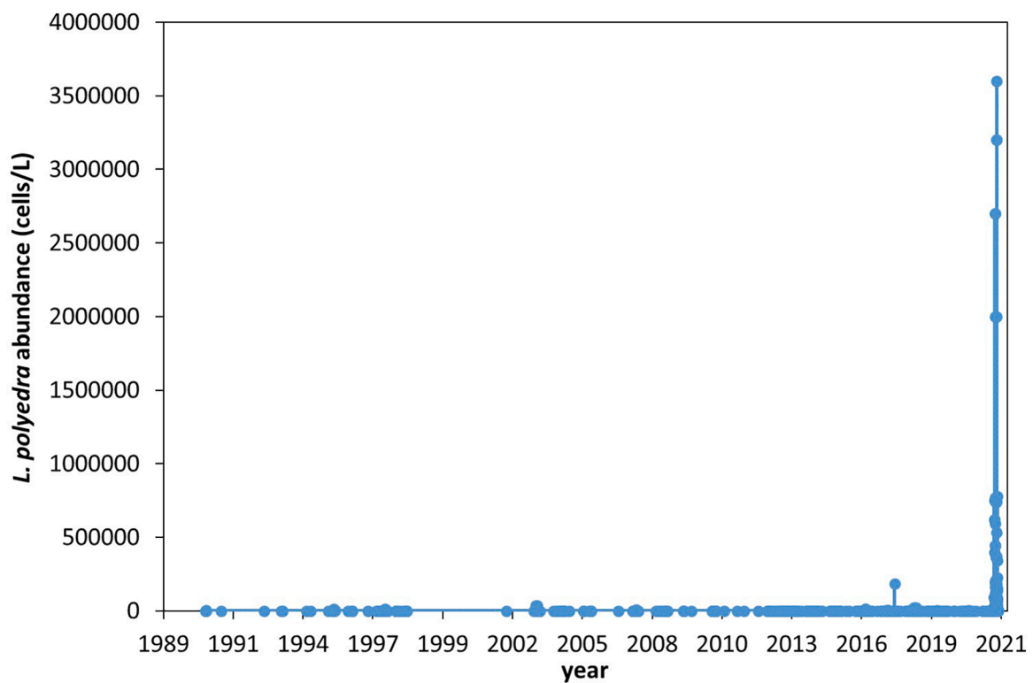
Fig. 17. Long-term record of L. polyedra concentrations (cells/L) recorded along the French Atlantic and Manche since 1990, extracted from the REPHY dataset (REPHY, 2022).
