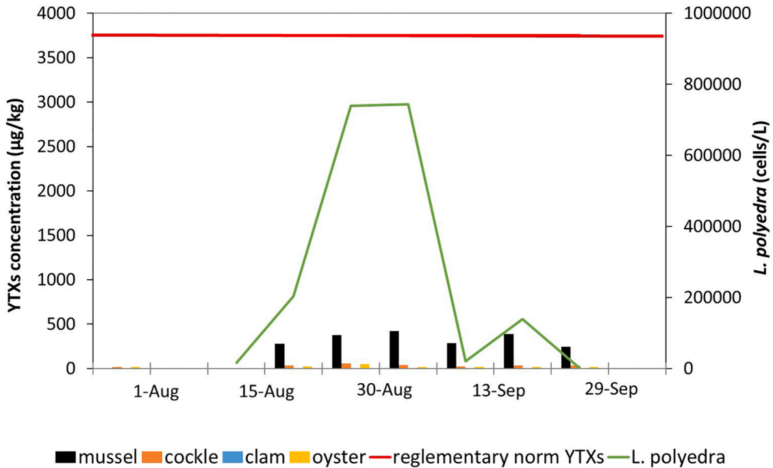
Fig. 14. YTX concentrations (µg/kg) measured in mussels and other shellfish and L. polyedra concentrations (cells/L) at Le Croisic (CR). Reglementary norm is indicated.
