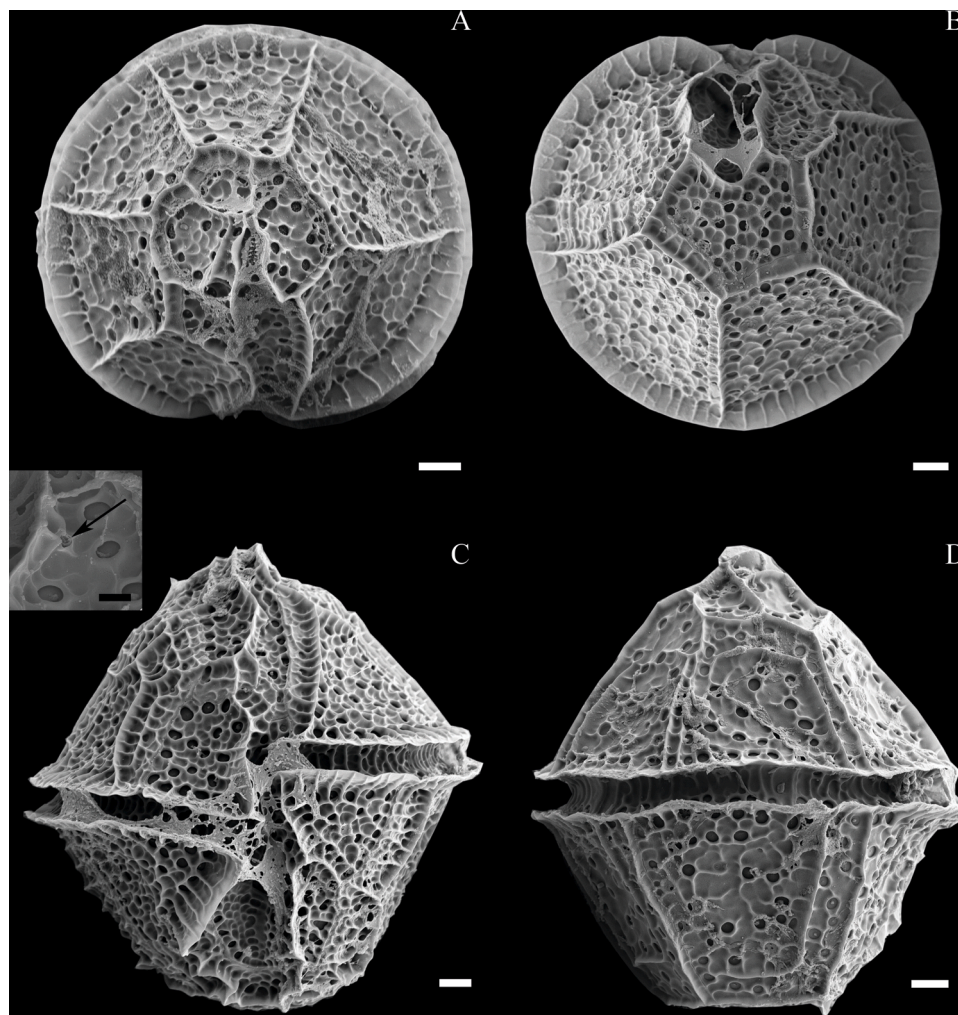
Fig. 11. Scanning electron micrographs of L. polyedra from Kervoyal (KE). (A) Apical view. (B) Antapical view. (C) Ventral view and detail of other cell showing presence of ventral pore (denoted by black arrow). (D) Dorsal view. All scale bars = 3 \mu m.
