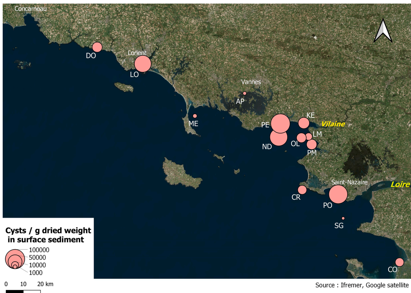
Fig. 15. Cyst concentrations in surface sediments (cysts/g dried weight) at the end of winter 2021/2022. AP = Anse de Pen Men, CO = Coupelasse, CR = Le Croisic, DO = Doëlan, KE = Kervoyal, LM = Le Maresclé, LO = Lorient harbor, ME = Men er Roué, ND = Nord Dumet, PE = Pénerf, OL = Ouest Loscolo, PM = Pont Mahé, PO = Pornichet Port, SG = Saint Gildas.
