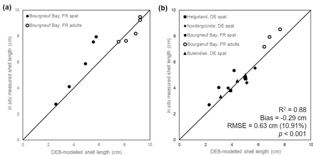
Fig. 6. (a) Calibration and (b) validation of the DEB half-saturation coefficient ( X_{ik} ).
